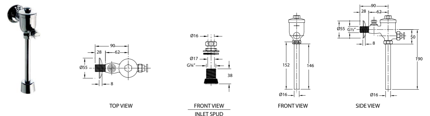
UF-3 | WGFA310106CP Exposed Urinal Flush Valve With Straight Pipe
